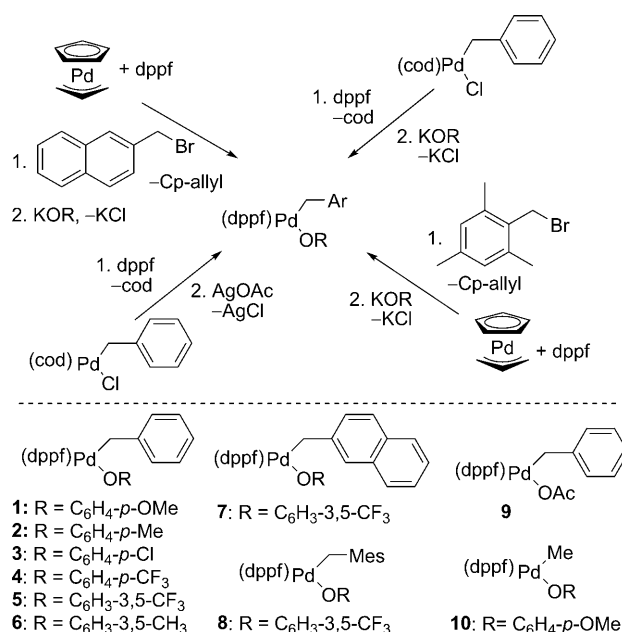
Scheme 1. Synthesis of palladium aryloxy complexes.
